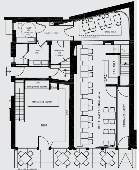
GROUND FLOOR PLAN OF nr.10 and nr.12 Lower Belgrave street
